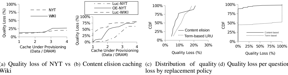
Figure 2: Cache under provisioning on quality loss.
